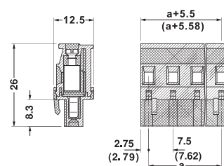
Pitch:7.62(7.5) mm
