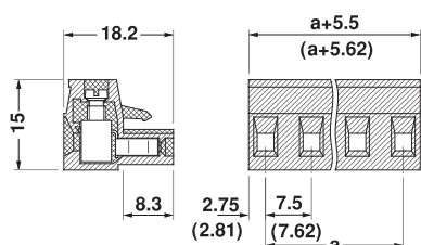
Pitch:7.62(7.5) mm
