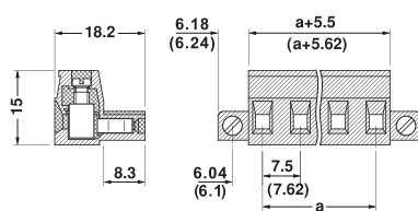
Pitch:7.62(7.5) mm
